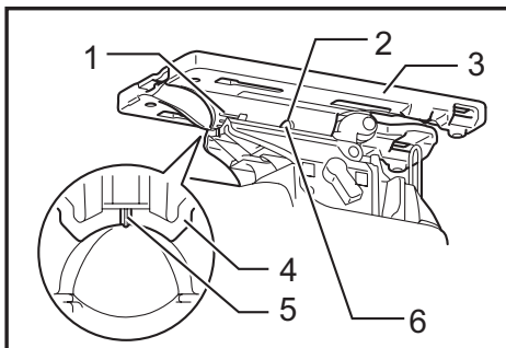
► 1. Graduation 2. Bevel slot 3. Base 4. Gear housing 5. V-notch 6. Bolt
